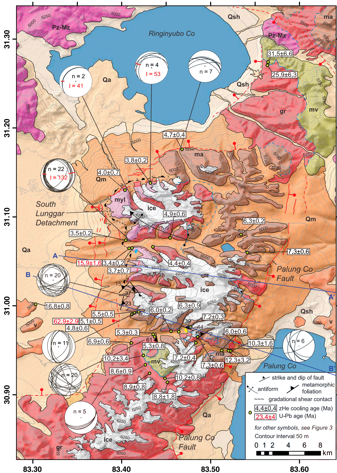
Figure 4. Geologic map of the South Lunggar rift. See Figure 3 for location. Note that cross-section lines A-A' and B-B' extend off the map to the east; see Figure 3 for full extent. On stereonet, “n” indicates the number of fault planes plotted, and “l” indicates the number of fault striations or stretching lineations measured; red lines indicate average orientation of lineations. Small blue and yellow arrows indicate position and direction field photographs (Figures 5c and 6c) were taken at. Zircon (U-Th)/He mean and 1\sigma errors are shown as well. Note the age for collocated samples SLE-SCTR-01 and SLE-SCTR-02 (30.94907°N, 83.52237) is the mean age for all aliquots.
